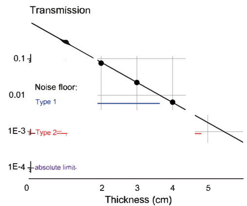
Thz transmission through paper stuck for the generators Type I and Type II
